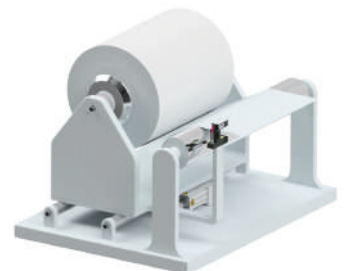
Guided winding
