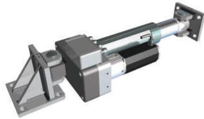
EMS 23 actuator Up to 295 mm stroke at max. 10,000 N
