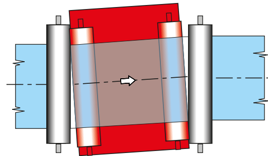
How the pivoting frame guide functions
