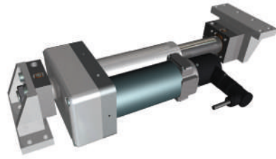
EMS 21 actuator Up to 195 mm stroke at max. 1,680 N
